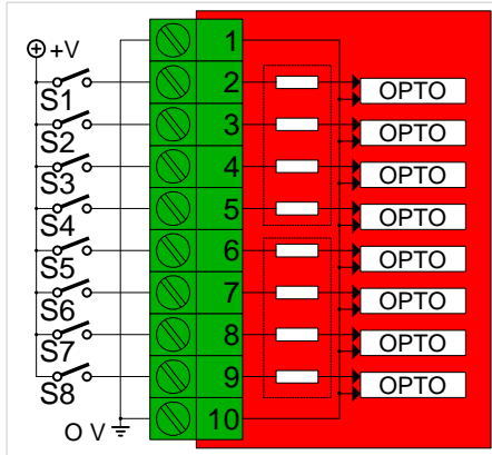
DI8-DC
