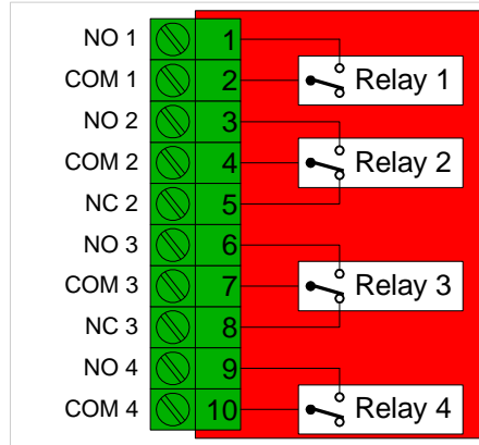
DO4-PR
